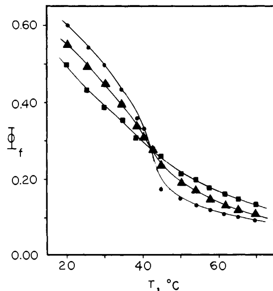
Figure 4. Effect of addition of cholesterol on the plot of quantum yield of fluorescence vs. temperature for S10A in DODAC vesicles.
