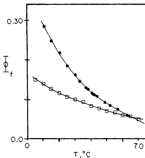
Figure 2. Quantum yield of fluorescence vs. temperature: \square , S6A in methylcyclohexane; \bullet , S16A in CTAC micelles.
