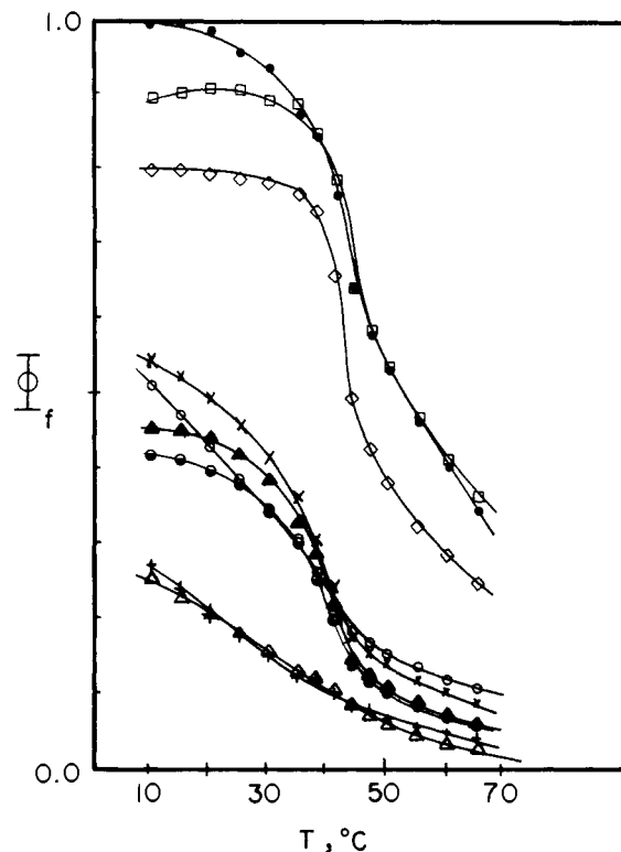
Figure 3. Quantum yield of fluorescence of surfactant stilbenes in dipalmitoyllecithin vesicles vs. temperature: \Delta , trans -stilbene; +, S4A; \bullet , S6A; \blacktriangle , S7A; \times , S10A; \circ , S12A; \diamond , 4S4; \square , 4S6A; \bullet , 6S4A.
