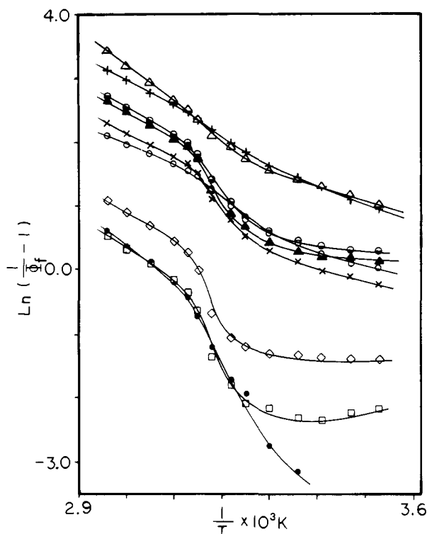
Figure 5. Arrhenius plot according to eq 6. Surfactant stilbenes in DPL; same symbols as Figure 3.
