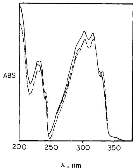
Figure 1. Effect of temperature ( ^{\circ}\text{C} ) on absorption spectrum of S10A in dipalmitoyllecithin vesicles: —, 60 and 45; ---, 35; - - -, 5.
